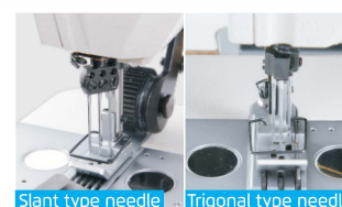
Two needle gauges (JK-8560G)
