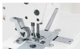
Rear puller
