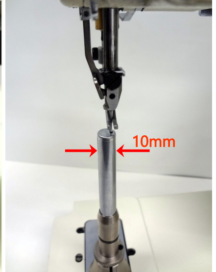
Suitable for sewing tubular part such as gloves' fingers
