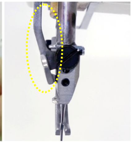
Needle thread catching system
